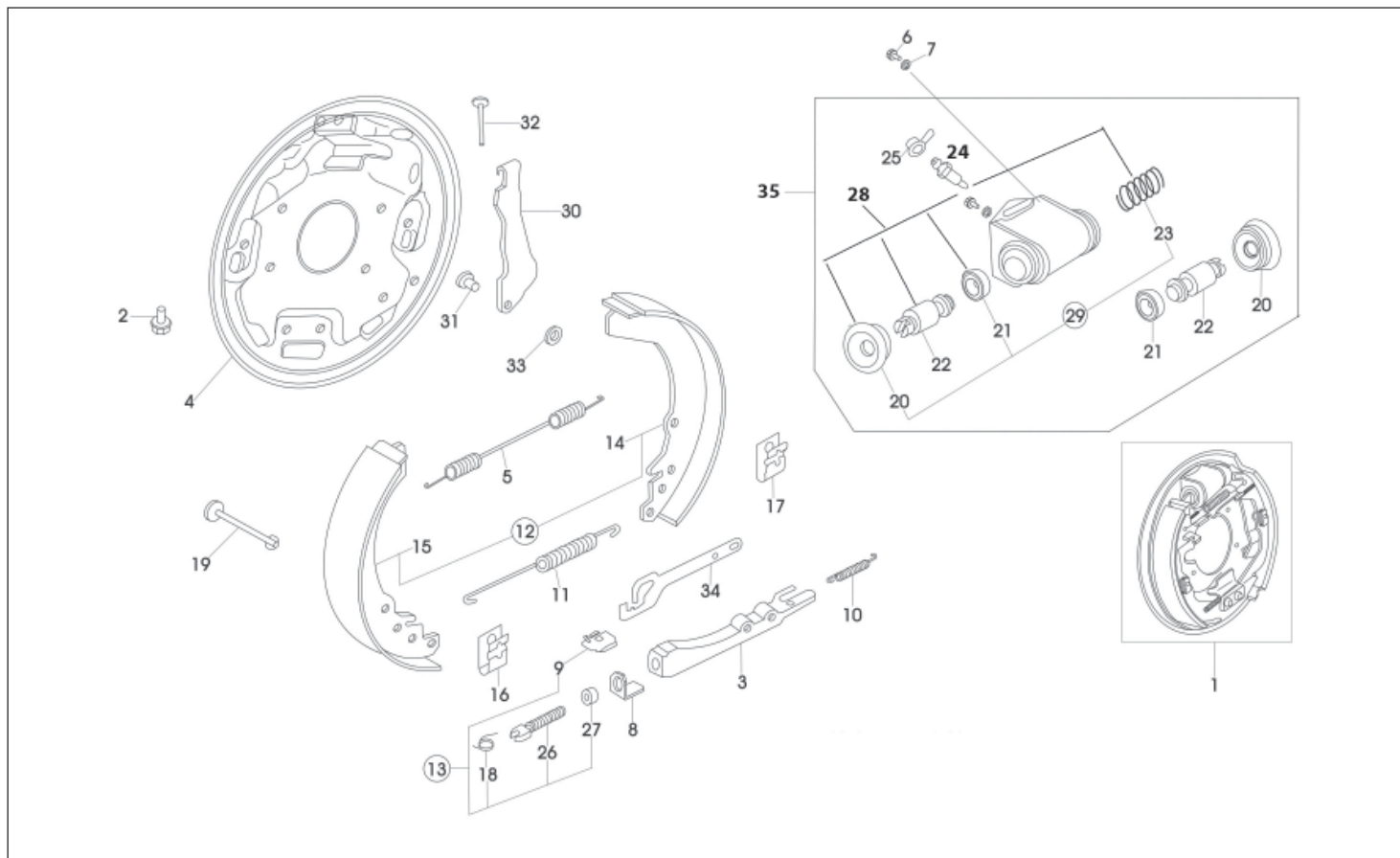
REAR BRAKE ASSEMBLY (KBX)
